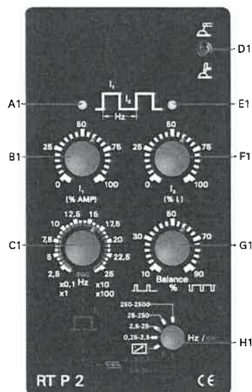
Abb.1: Handfernsteller RTP 2
