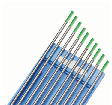
= rein Wolfram
