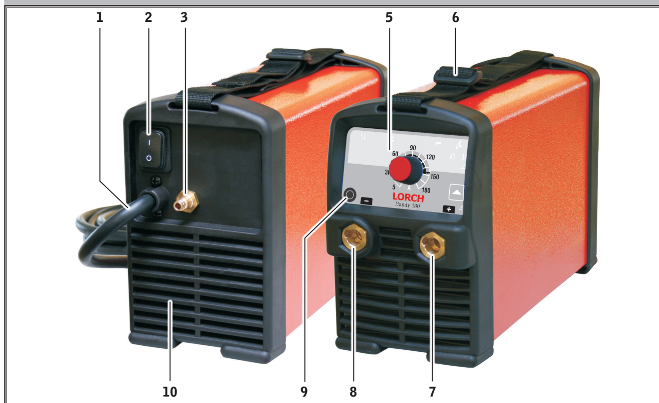
Abb. 1: Machine elements
