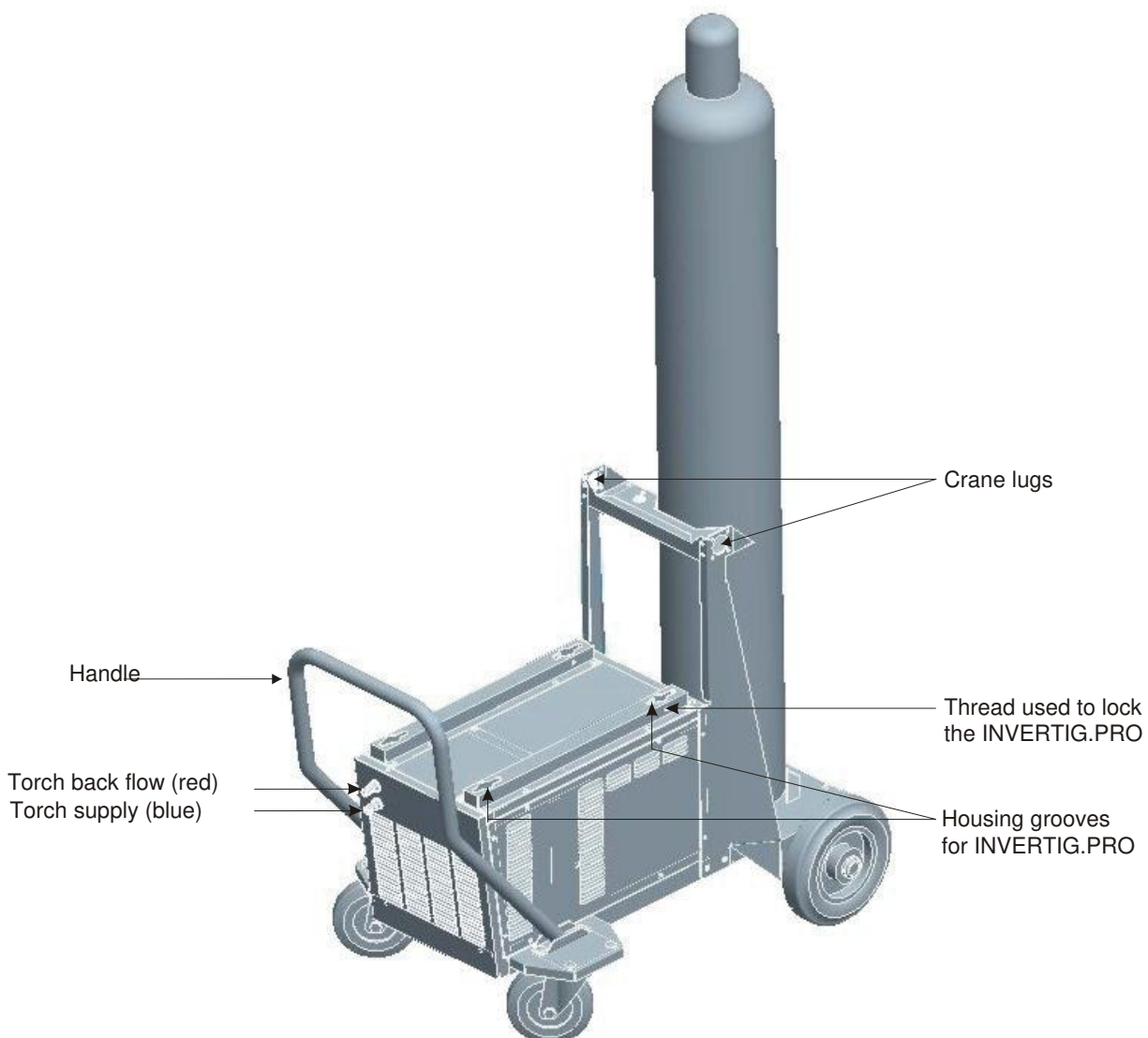
Figure 2: TIG – COOL CART 2000 with gas tank
