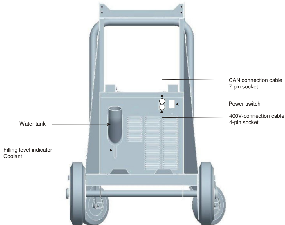
Figure 3: TIG - COOL CART 2000 view from behind
